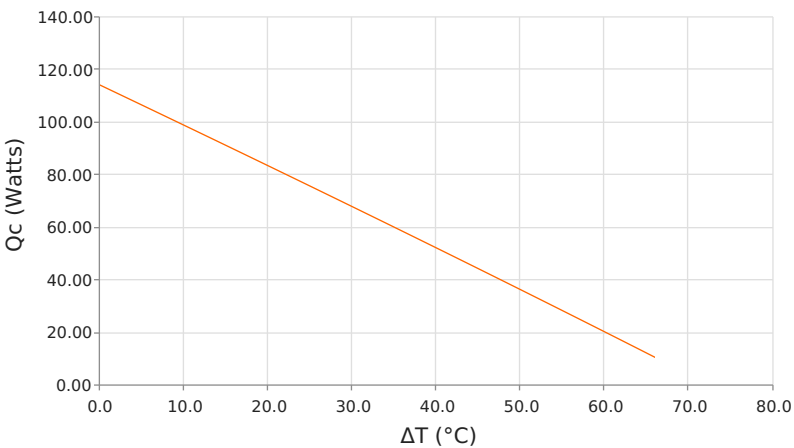
Heat Pumped at Cold Side ( Q_c ) T_{hot} = 35\text{ }^{\circ}\text{C} | operating = 12.1 Amps
