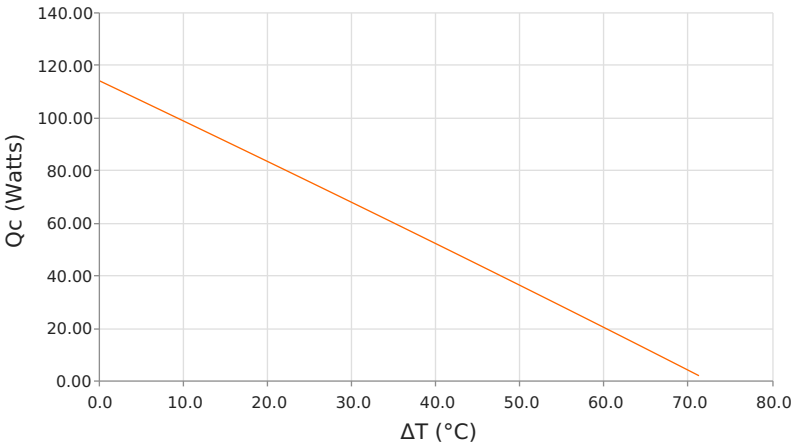
Heat Pumped at Cold Side ( Q_c ) T_{hot} = 35\text{ }^\circ\text{C} | i_{operating} = 12.1\text{ Amps}
