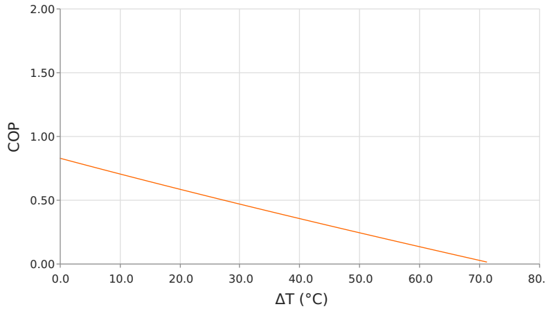
Coefficient of Performance (COP = Q_c/P_{in} ) T_{hot} = 35^\circ\text{C} | operating = 3.3 Amps
