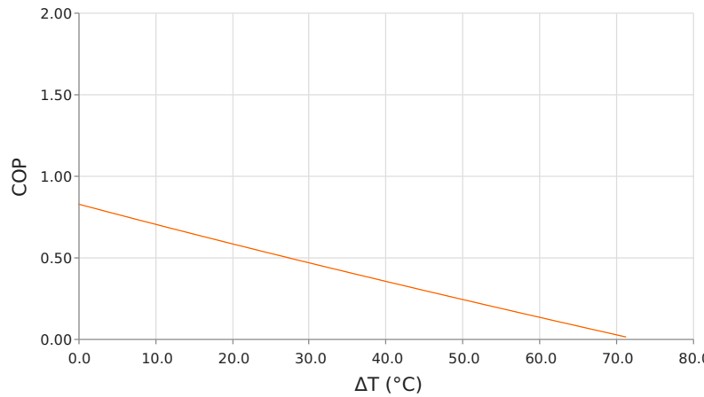
Coefficient of Performance ( COP = Q_c/P_{in} ) T_{hot} = 35^\circ C | operating = 3.3 Amps
