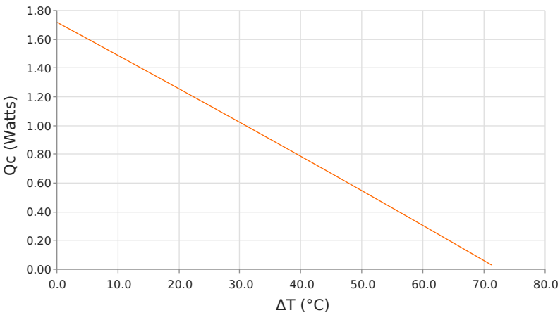
Heat Pumped at Cold Side ( Q_c ) T_{hot} = 35^\circ C | operating = 3.3 Amps
