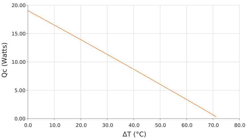
Heat Pumped at Cold Side ( Q_c ) T_{hot} = 35^\circ\text{C} | operating = 7.3 Amps
