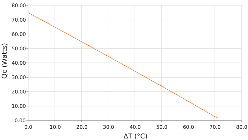
Heat Pumped at Cold Side ( Q_c ) T_{hot} = 35^\circ\text{C} | operating = 5.1 Amps
