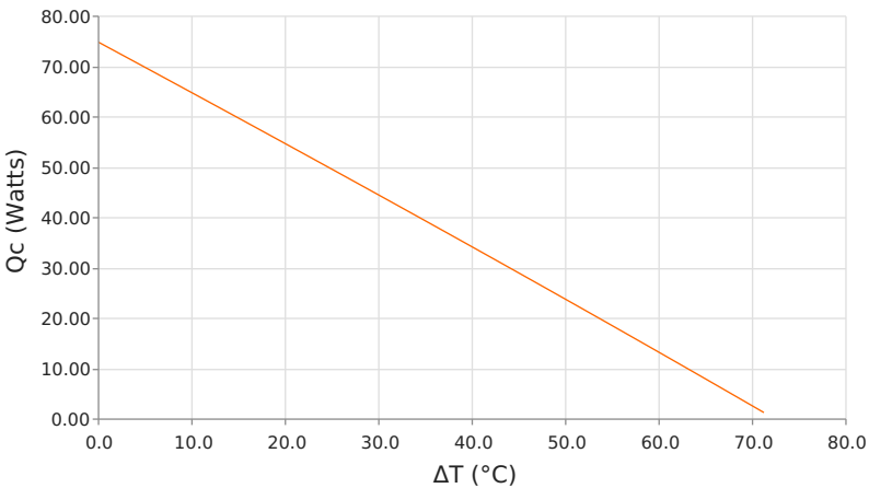
Heat Pumped at Cold Side ( Q_c ) T_{hot} = 35^\circ\text{C} | operating = 5.1 Amps
