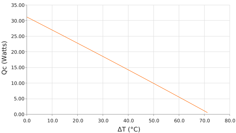
Heat Pumped at Cold Side ( Q_c ) T_{hot} = 35\text{ }^{\circ}\text{C} | operating = 3.3 Amps
