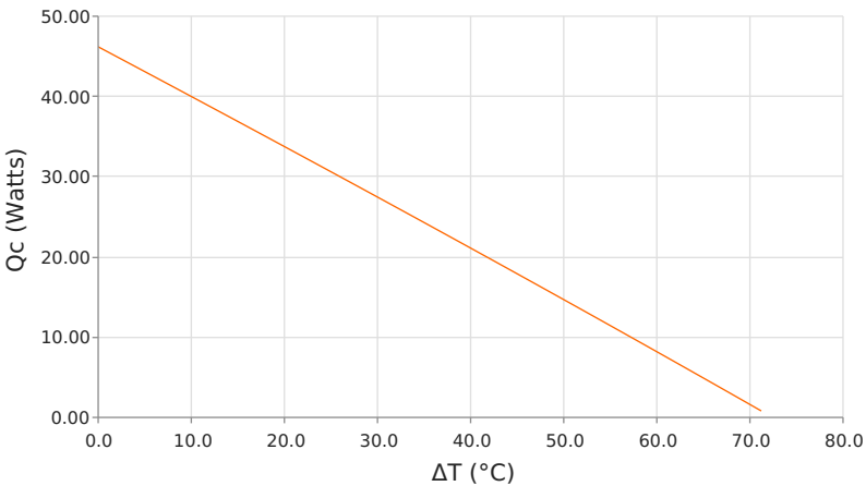
Heat Pumped at Cold Side ( Q_c ) T_{hot} = 35^\circ\text{C} | operating = 3.9 Amps
