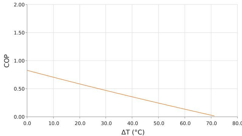
Coefficient of Performance (COP = Q_c/P_{in} ) T_{hot} = 35^\circ\text{C} | operating = 3.9 Amps
