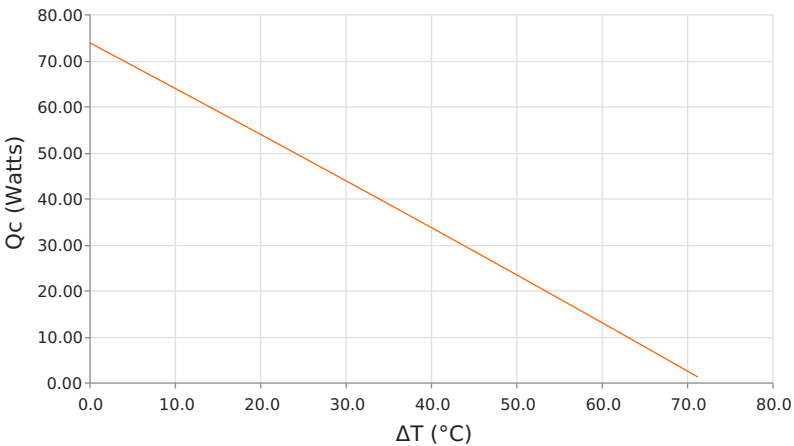
Heat Pumped at Cold Side ( Q_c ) T_{hot} = 35\text{ }^{\circ}\text{C} | operating = 6.2 Amps
