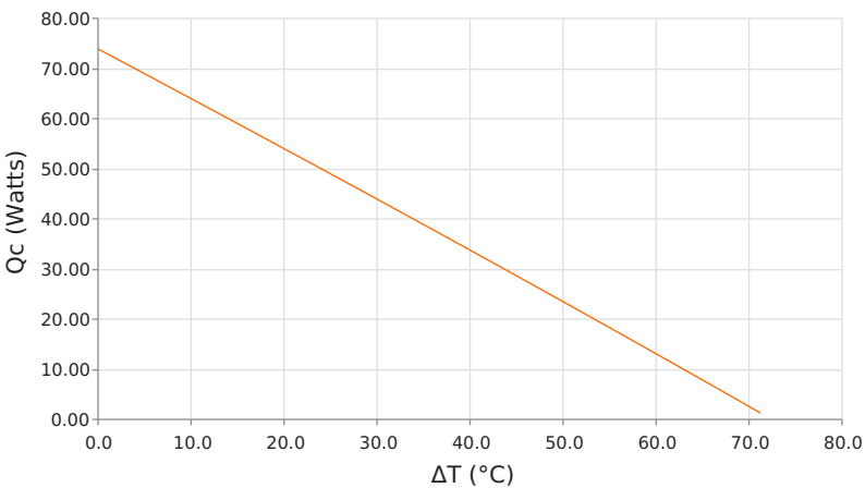
Heat Pumped at Cold Side ( Q_c ) T_{hot} = 35^\circ C | operating = 6.2 Amps
