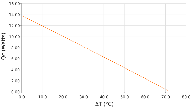
Heat Pumped at Cold Side ( Q_c ) T_{hot} = 35^\circ\text{C} | operating = 2.6 Amps
