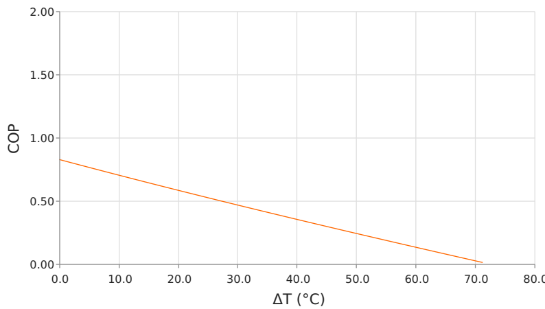
Coefficient of Performance (COP = Qc/Pin) Thot = 35 °C | Ioperating = 2.6 Amps
