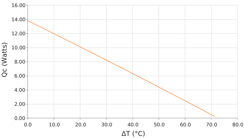
Heat Pumped at Cold Side (Qc) Thot = 35 °C | Ioperating = 2.6 Amps
