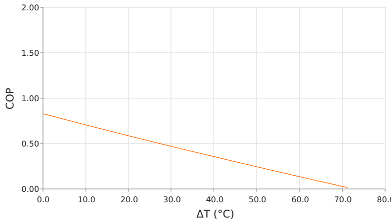
Coefficient of Performance (COP = Qc/Pin) Thot = 35 °C | Ioperating = 3.4 Amps
