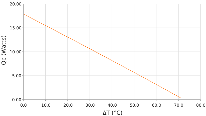
Heat Pumped at Cold Side (Qc) Thot = 35 °C | Ioperating = 3.4 Amps
