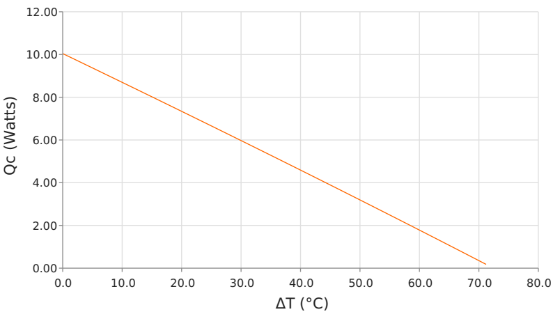
Heat Pumped at Cold Side ( Q_c ) T_{hot} = 35\text{ }^{\circ}\text{C} | operating = 2.1 Amps
