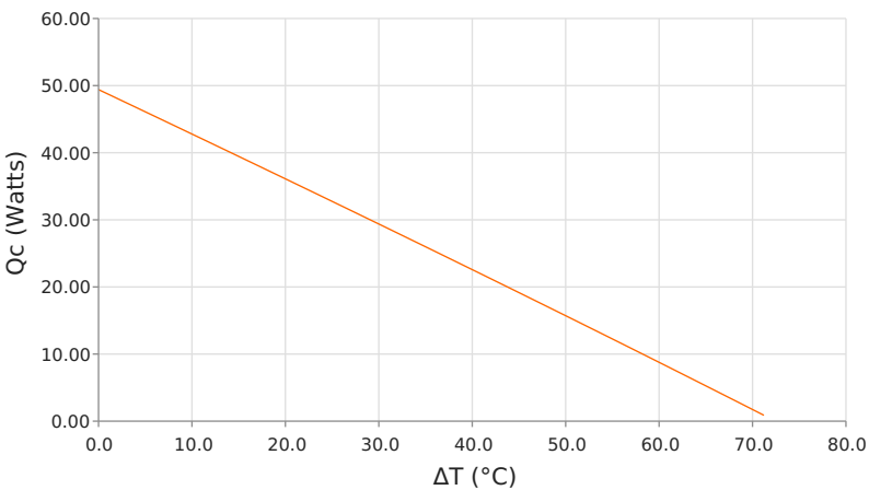
Heat Pumped at Cold Side ( Q_c ) T_{hot} = 35^\circ C | operating = 2.6 Amps
