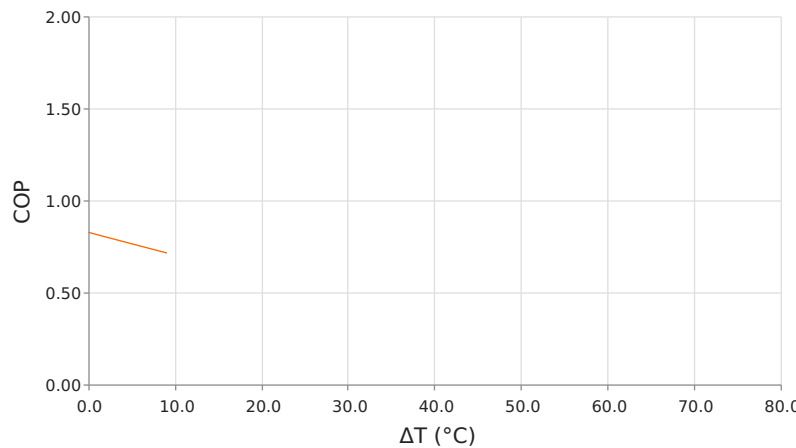
Coefficient of Performance ( COP = Q_c/P_{in} ) T_{hot} = 35\text{ }^{\circ}\text{C} | operating = 2.6 Amps
