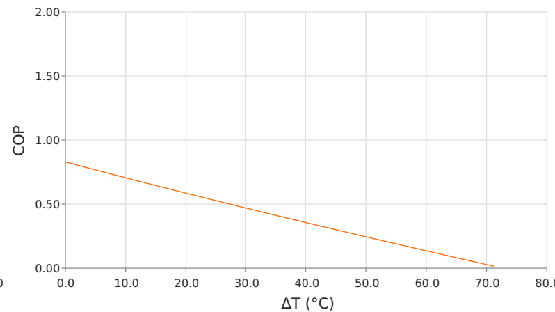
Coefficient of Performance (COP = Q_c/P_{in} ) T_{hot} = 35^\circ\text{C} | operating = 5.2 Amps
