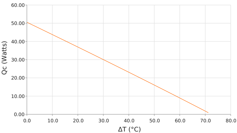
Heat Pumped at Cold Side ( Q_c ) T_{hot} = 35^\circ\text{C} | operating = 5.2 Amps
