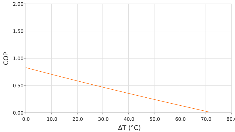
Coefficient of Performance (COP = Qc/Pin) Thot = 35 °C | Ioperating = 1.8 Amps
