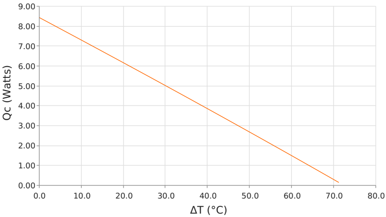
Heat Pumped at Cold Side (Qc) Thot = 35 °C | Ioperating = 1.8 Amps
